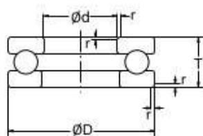
Boundary dimensions of single-direction thrust ball bearings
