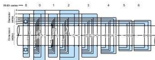
Comparison of the cross sections of radial bearings (except tapered roller bearings) for various dimension series
